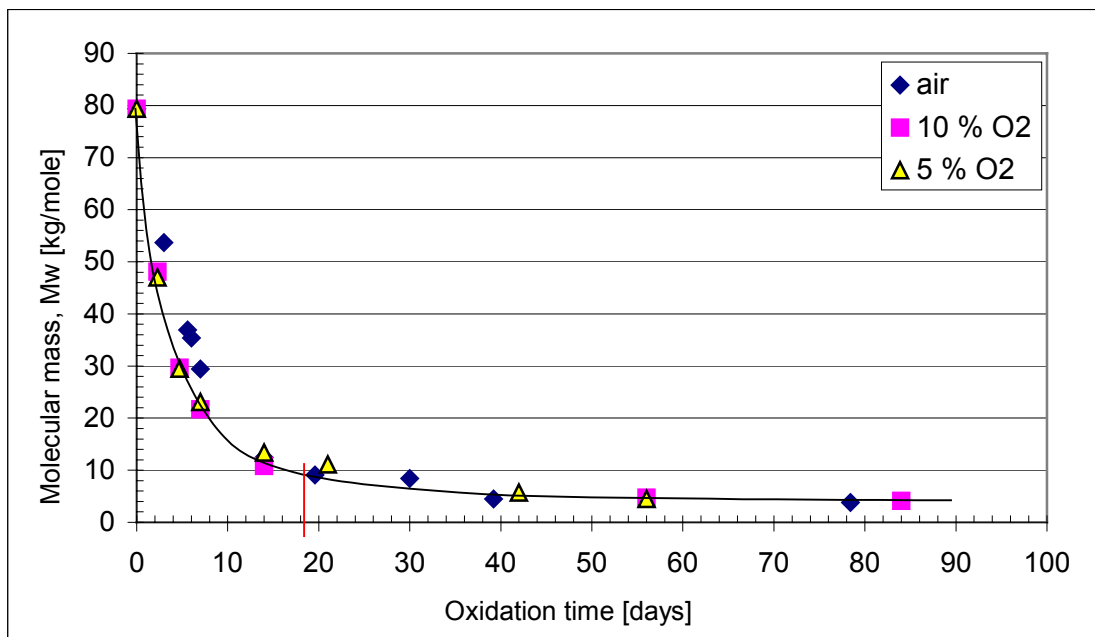
Figure 2. Effect of oxygen content on the rate of degradation of the AF 10 material. Superposition analysis by shifting data to 60 °C.
