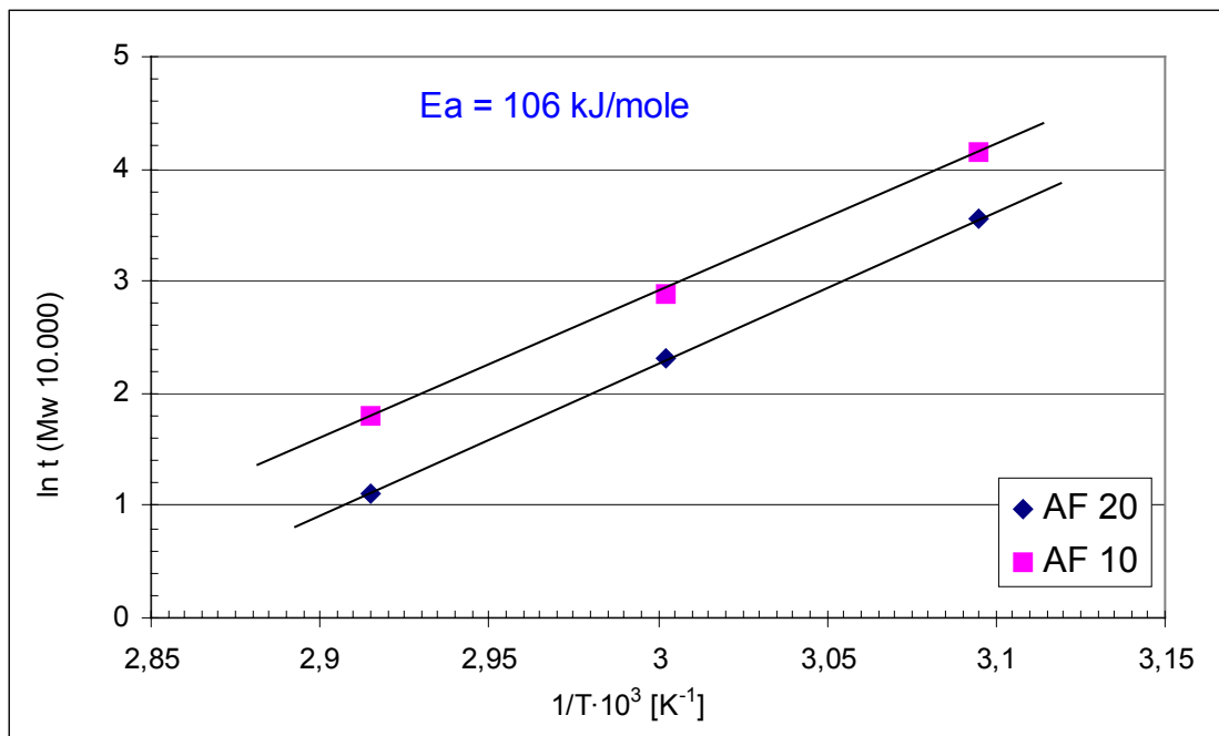
Figure 4. Arrhenius plot
