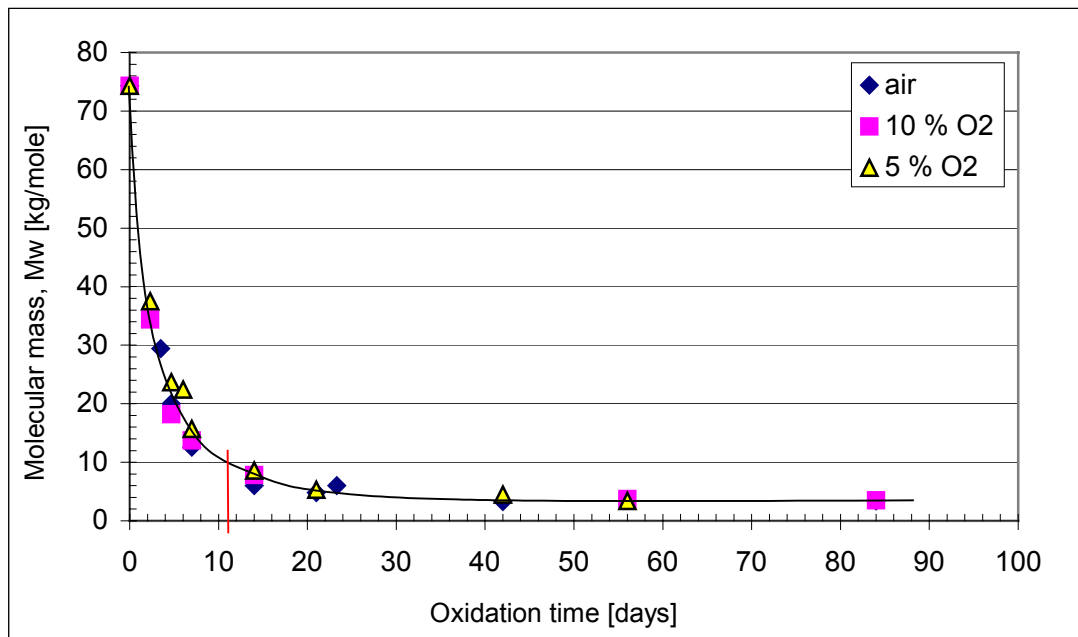
Figure 3. Effect of oxygen content on the rate of degradation of the AF 20 material. Superposition analysis by shifting data to 60 °C.
