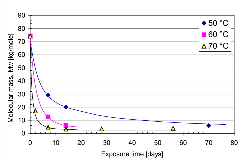
Figure 1. Change of molecular mass (Mw) of the AF 20 material with exposure time at various temperatures in air.
